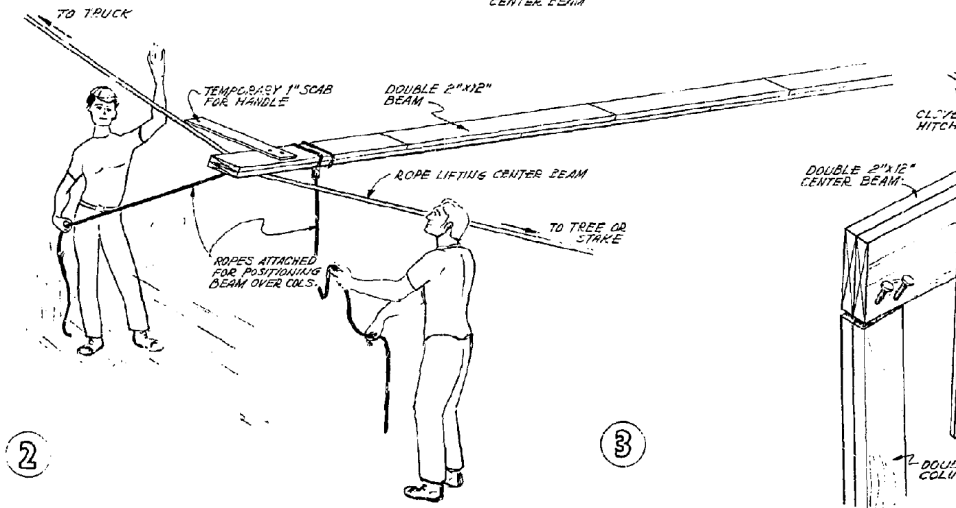
Fig. A-9.1. Rigid-Frame, Continuous Vent, Semiburied Shelter, P and Elevation.
